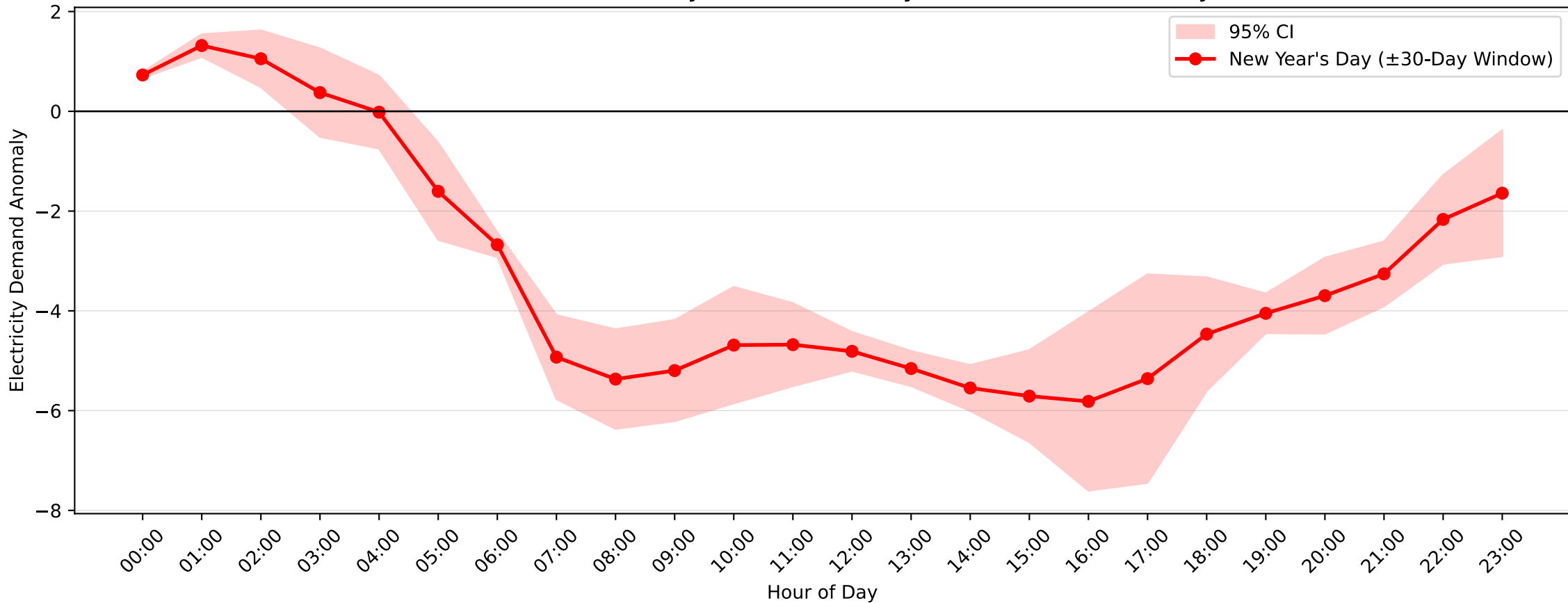
Hunters Hill Demand Anomaly: New Year's Day (2016-2017, \pm 30 -Day Window)
