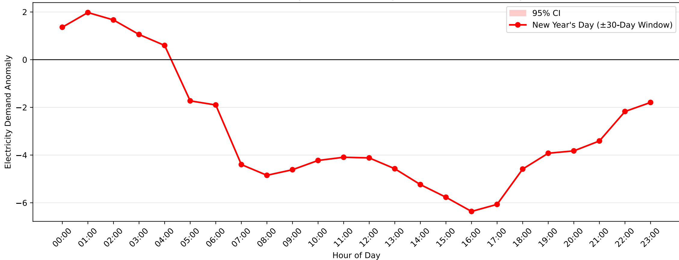
Hunters Hill Demand Anomaly: New Year's Day (2017-2018, \pm 30 -Day Window)
