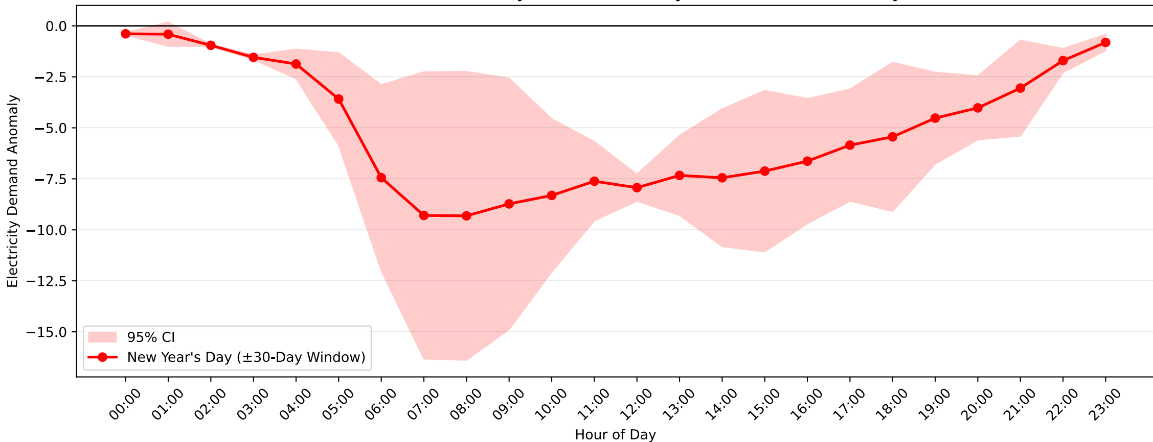
Hunters Hill Demand Anomaly: New Year's Day (2004–2005, \pm 30 -Day Window)
