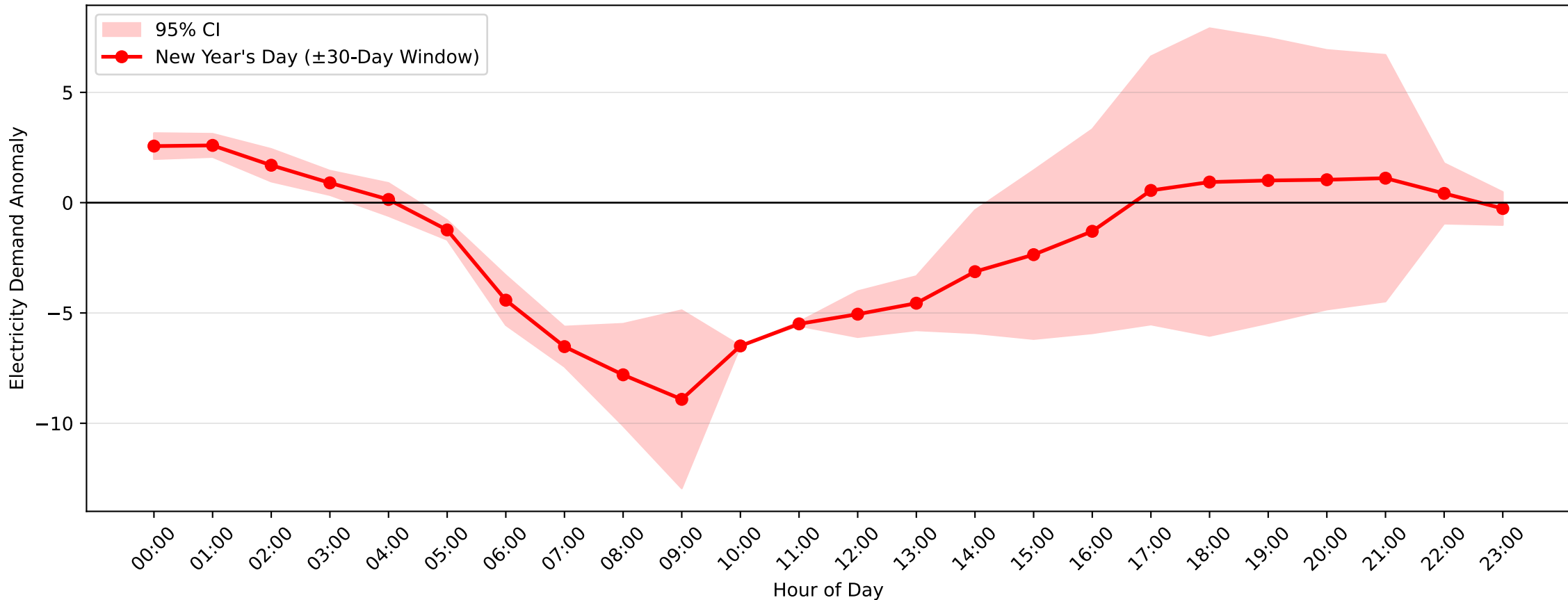
Hunters Hill Demand Anomaly: New Year's Day (2008-2009, \pm 30 -Day Window)
