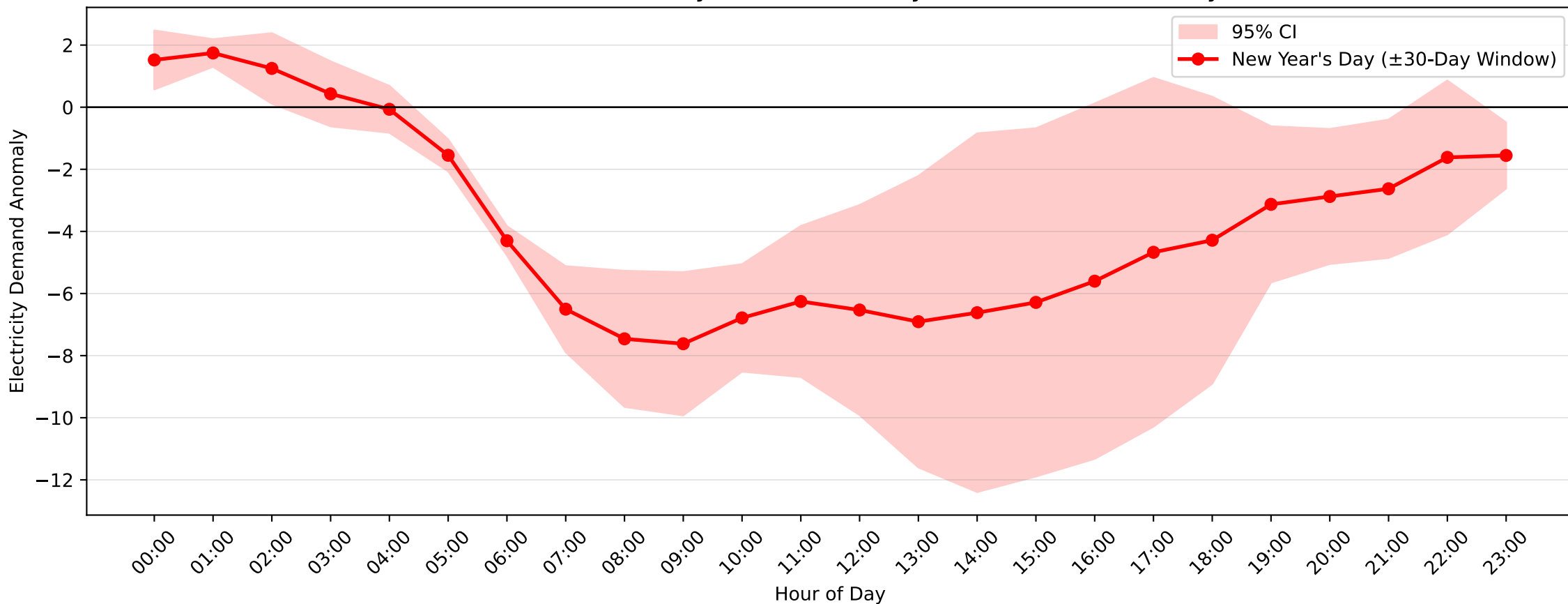
Hunters Hill Demand Anomaly: New Year's Day (2007-2008, \pm 30 -Day Window)
