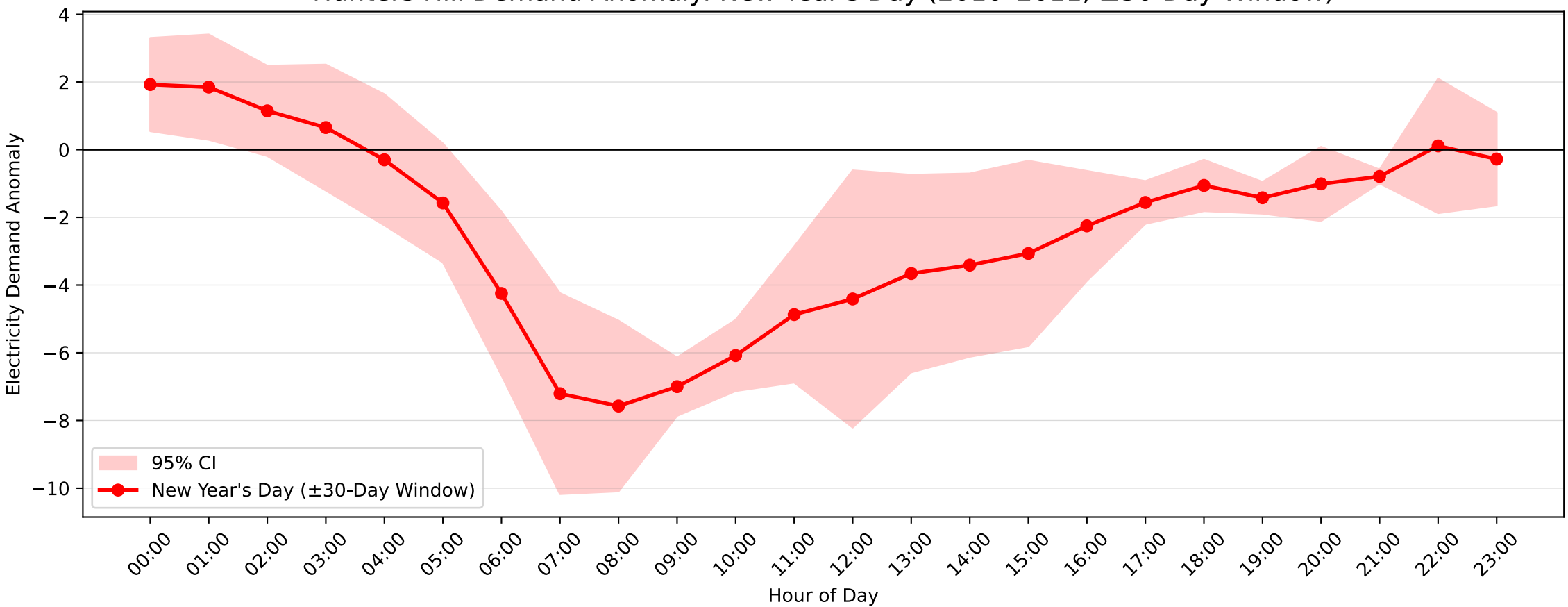
Hunters Hill Demand Anomaly: New Year's Day (2010-2011, \pm 30 -Day Window)
