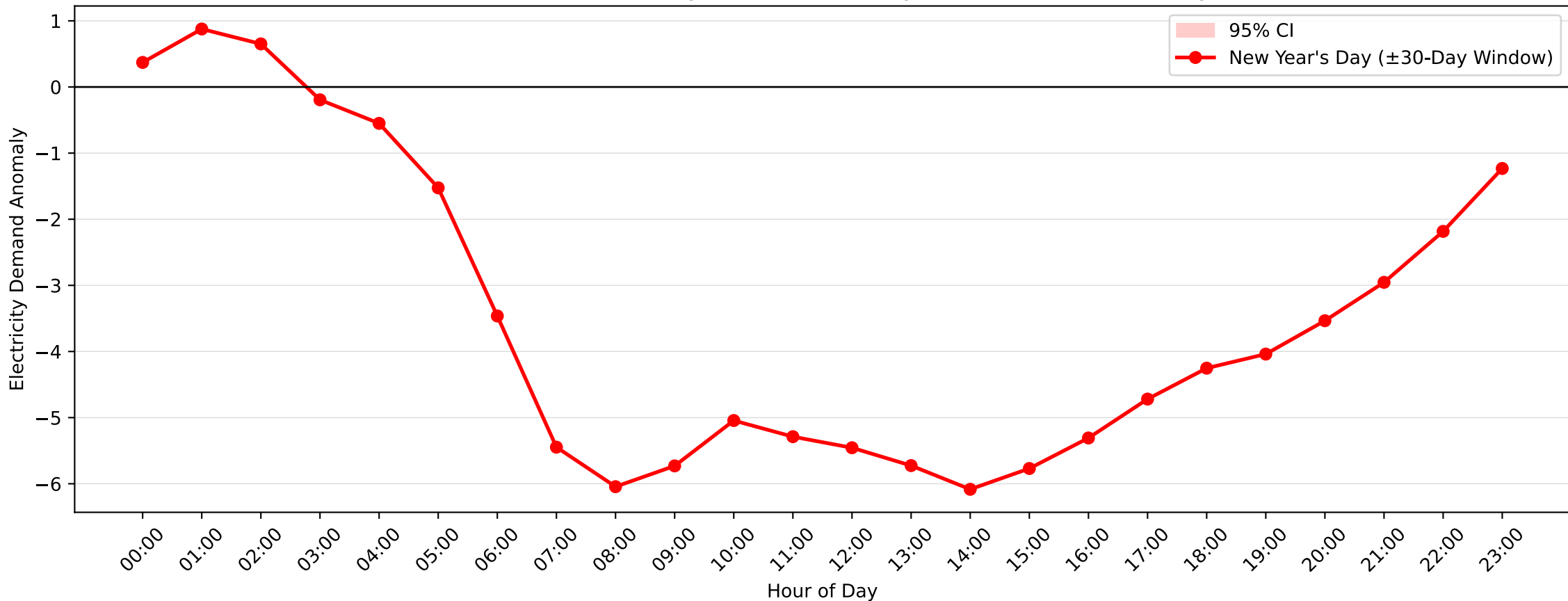
Hunters Hill Demand Anomaly: New Year's Day (2015-2016, \pm 30 -Day Window)
