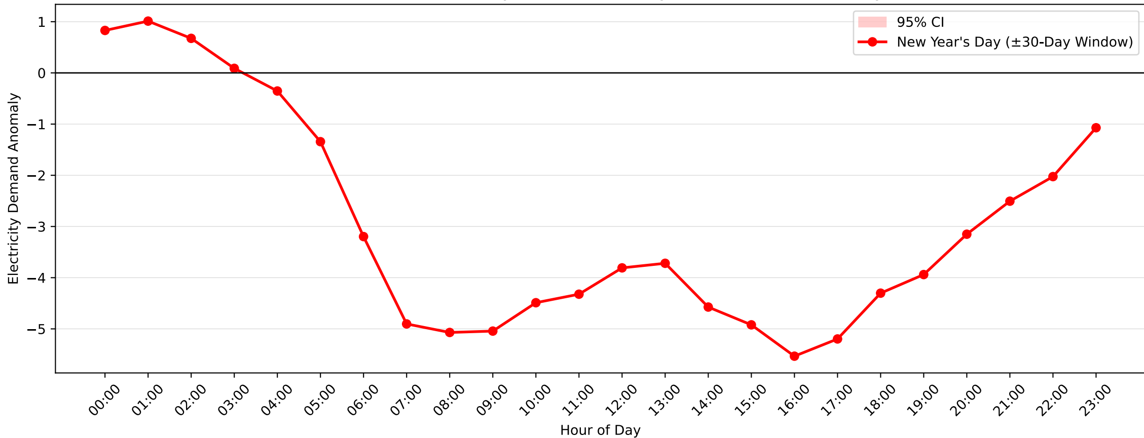
Hunters Hill Demand Anomaly: New Year's Day (2014-2015, \pm 30 -Day Window)
