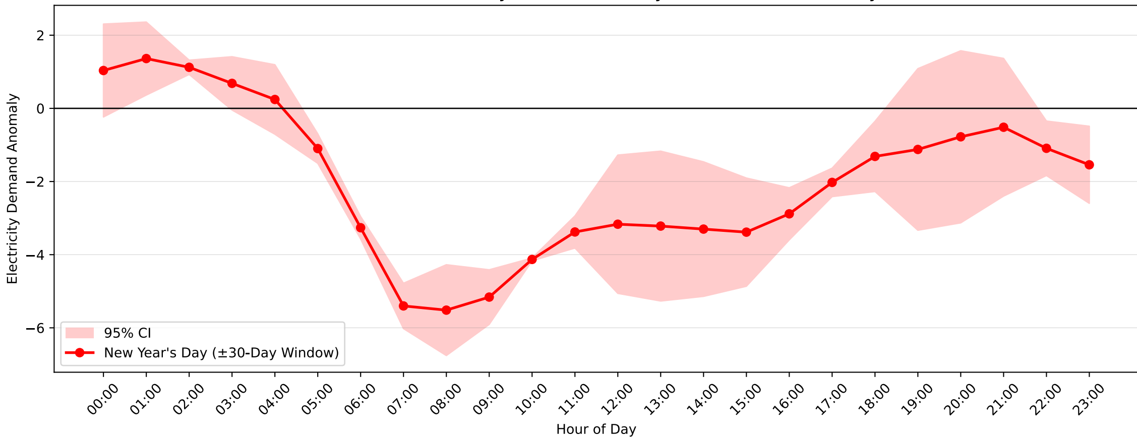
Hunters Hill Demand Anomaly: New Year's Day (2012-2013, \pm 30 -Day Window)
