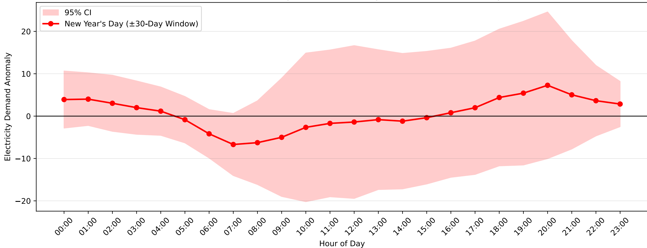
Hunters Hill Demand Anomaly: New Year's Day (2005-2006, \pm 30 -Day Window)
