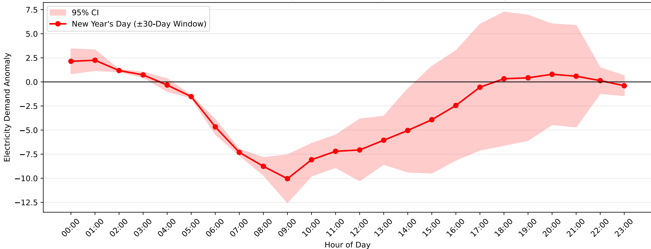
Hunters Hill Demand Anomaly: New Year's Day (2009–2010, \pm 30 -Day Window)
