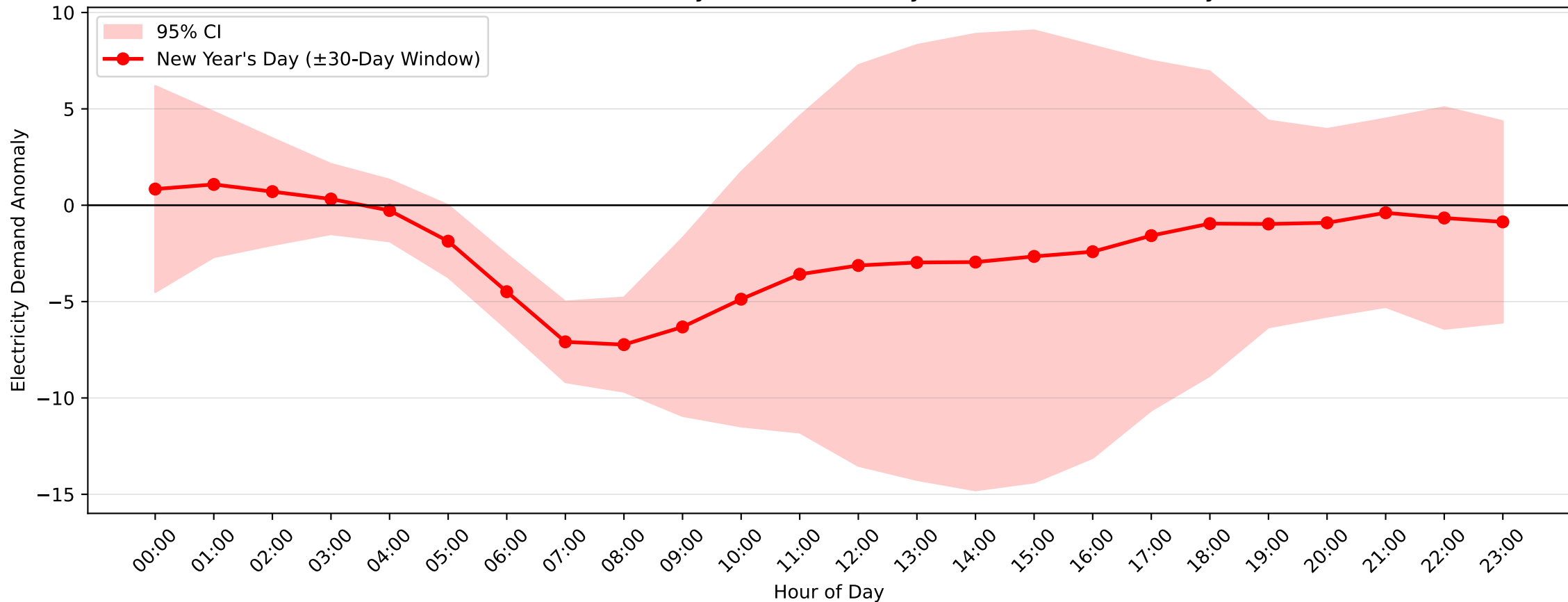
Hunters Hill Demand Anomaly: New Year's Day (2011-2012, \pm 30 -Day Window)
