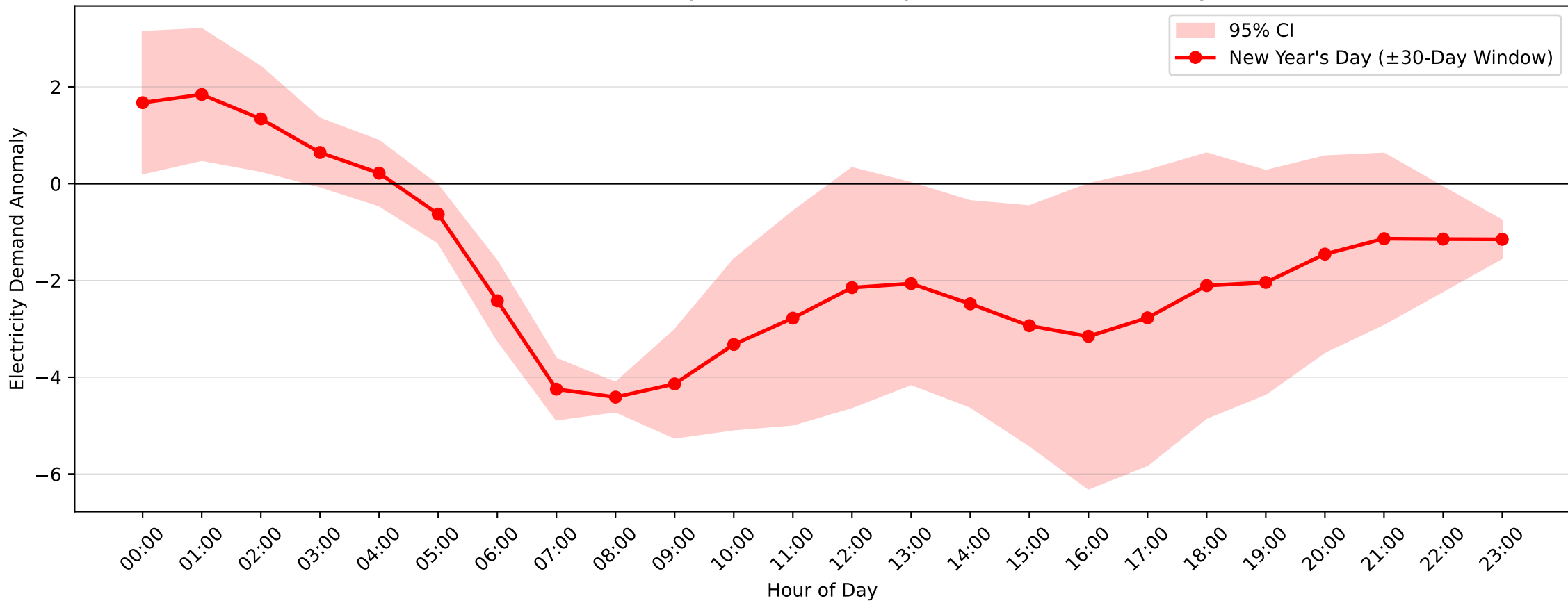
Hunters Hill Demand Anomaly: New Year's Day (2013-2014, \pm 30 -Day Window)
